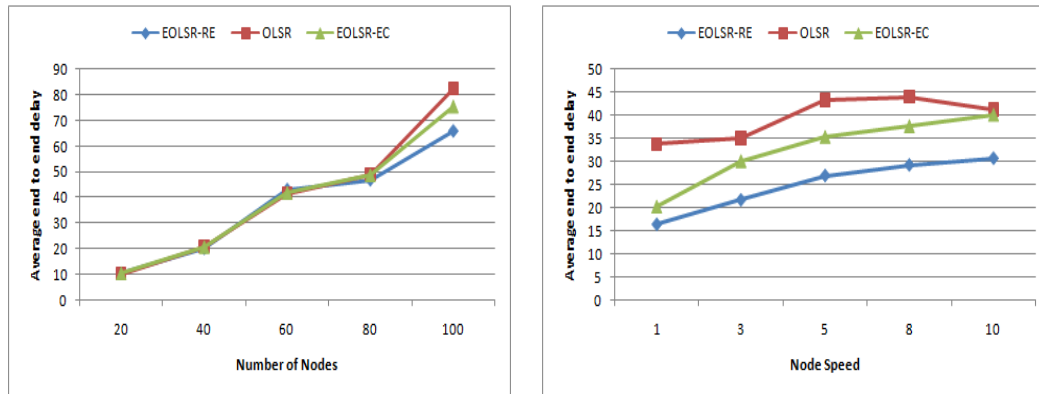
Figure 10: Impact of Variation of Number of Nodes and Node Speed on Average end to end delay
