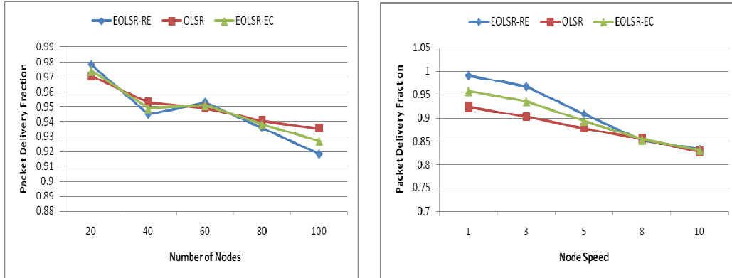
Figure 11: Impact of Variation of Number of Nodes and Node Speed on Packet Delivery Fraction
