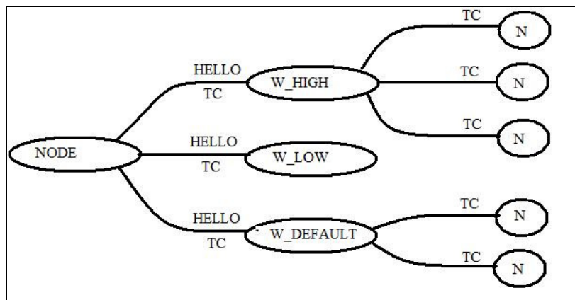
Figure 2. Selection of MPR and Broadcasting TC packets
