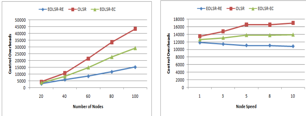
Figure 13: Impact of Variation of Number of Nodes and Node Speed on Control Overheads
