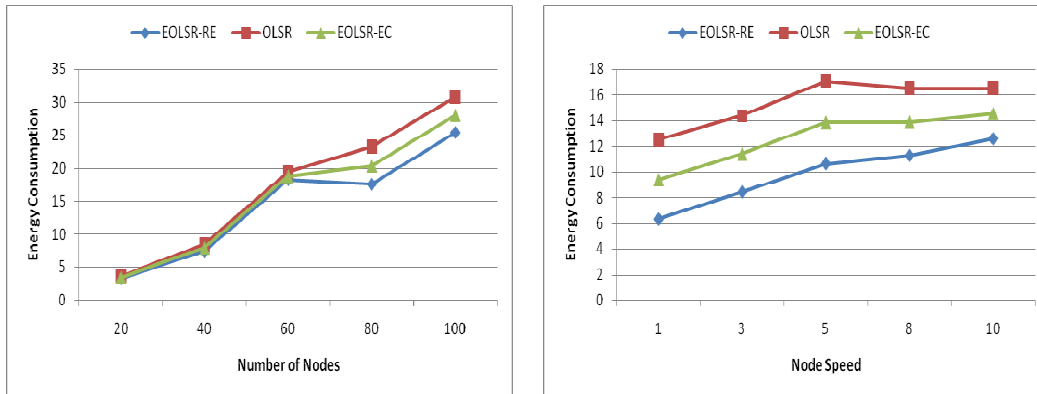
Figure 12: Impact of Variation of Number of Nodes and Node Speed on Energy Consumption
